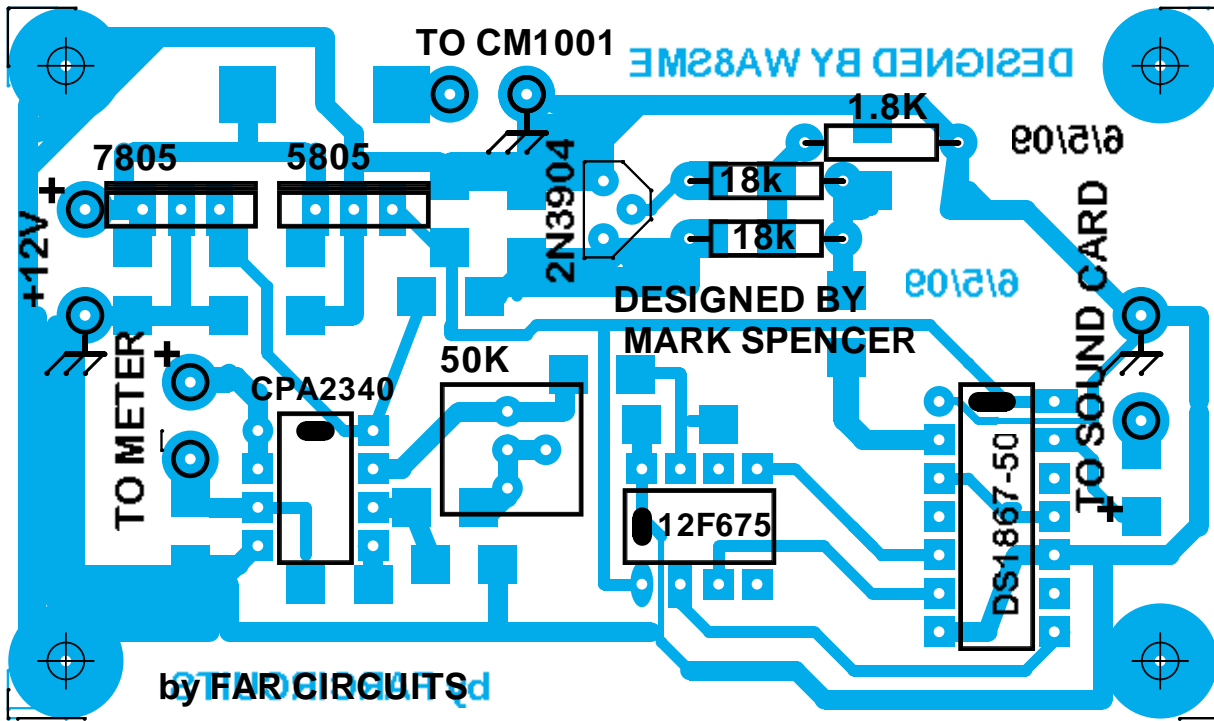
TOP COMPONENT LAYER 3.15" BY 1.85"
